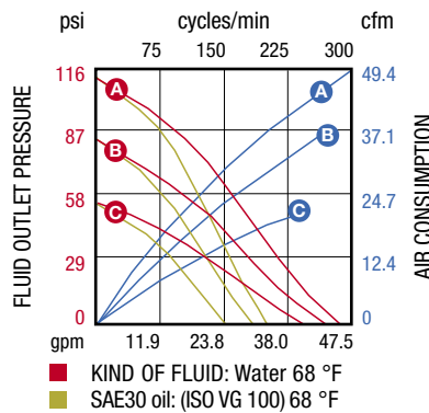
PUMP AIR FEEDING PRESSURE A 116 psi B 87 psi C 58 psi
