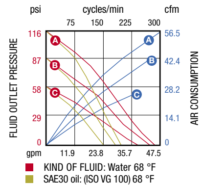
PUMP AIR FEEDING PRESSURE B 87 psi C 58 psi
